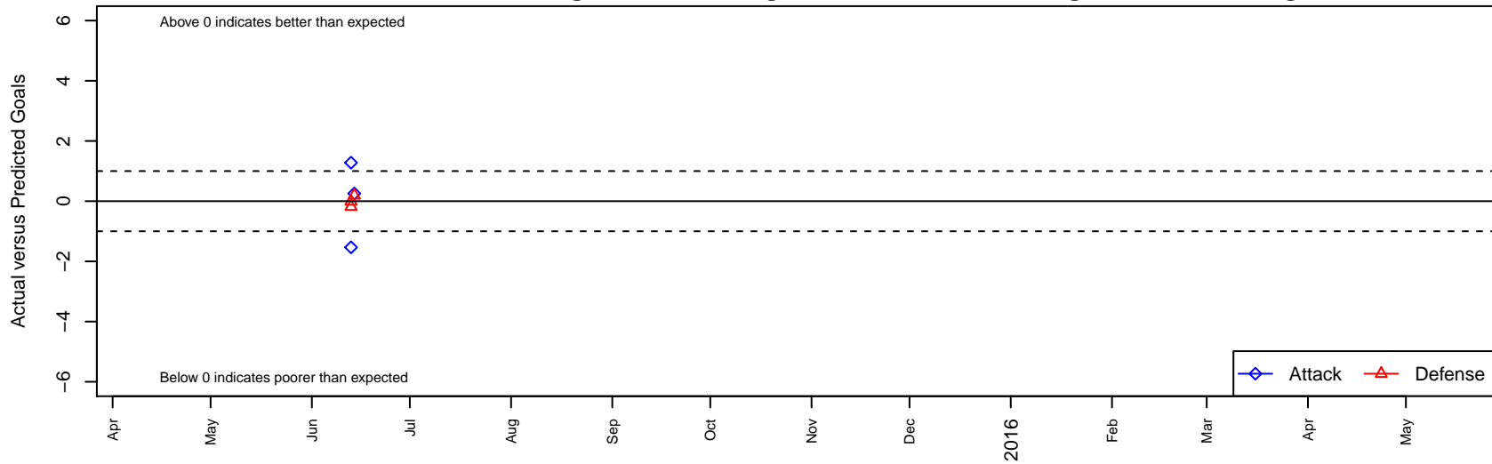
NSGS Metro Renegades 2001G Dots are actual minus expected GF (blue circles) and GA (red triangles). Blue line is smoothed change in attack strength. Red is smoothed change in defense strength.
